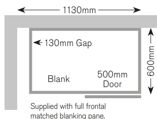
2100mm high CNLU106/A/F 2276mm high CNLU10623/A/F
