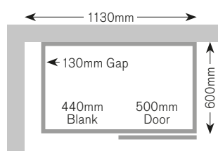
Full Height CB106FAFP Drawer Line CB106DAFP
