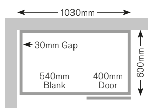
Full Height CB106FBFP Drawer Line CB106DBFP
