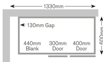
Full Height CB126FFFP Drawer Line CB126DFFP
