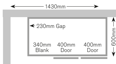
Full Height CB126FEFP Drawer Line CB126DEFP
