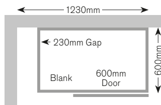
2100mm high CNLU106C/A/F 2276mm high CNLU10623C/A/F
