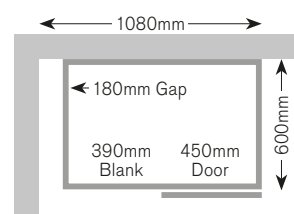
Full Height CB96FAFP Drawer Line CB96DAFP
